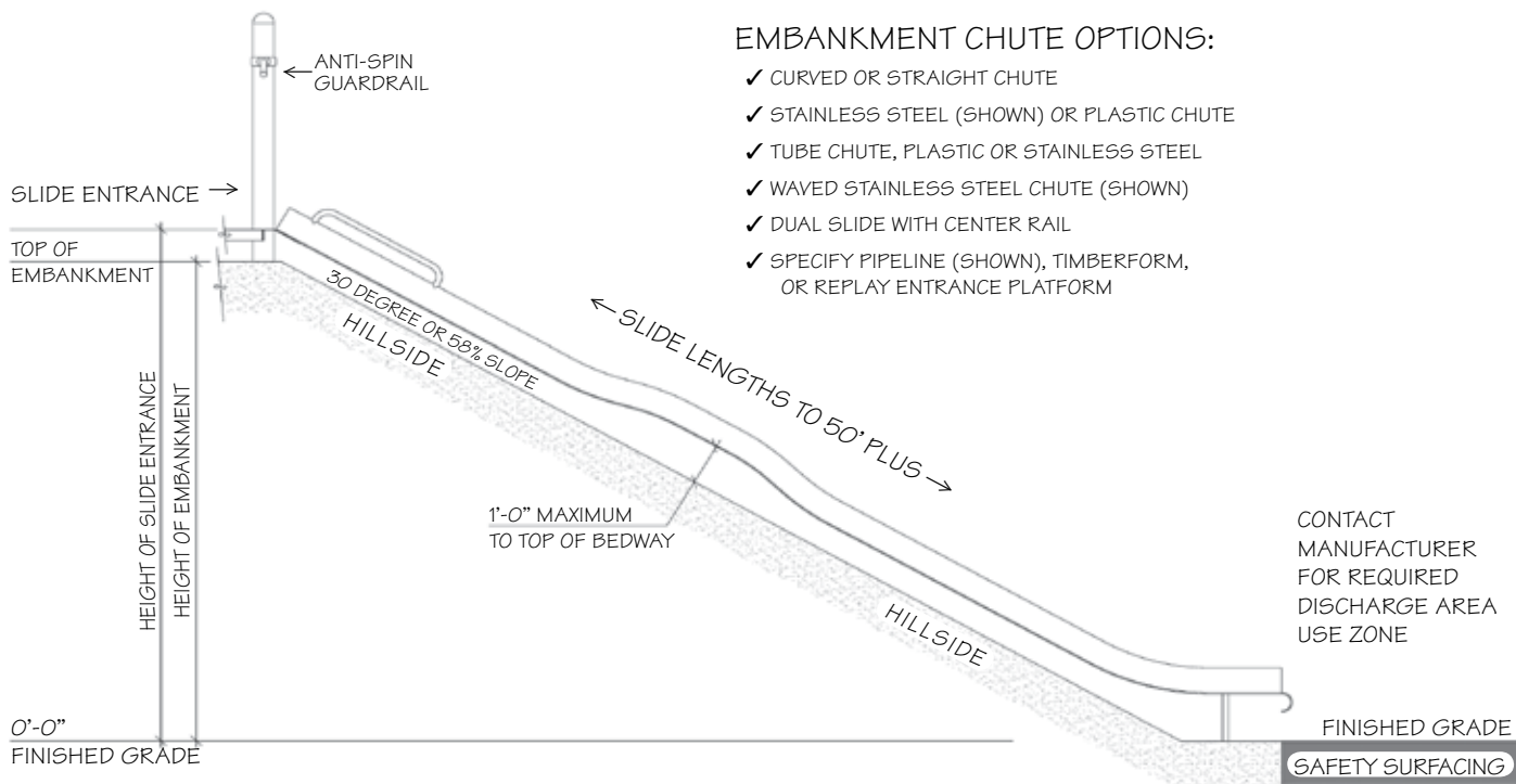
TYPICAL EMBANKMENT SLIDE CHUTE— SIDE VIEW
