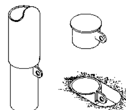
Removable Mount Option Detail
