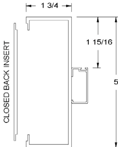
5-INCH FRAME WITH OPTIONAL INSERT
