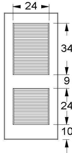
TOP AND BOTTOM LOUVER
