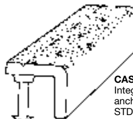
TYPE 150 1\frac{1}{2} " x 1\frac{1}{2} " x \frac{3}{8} " (38.1 mm x 38.1 mm x 9.53 mm) Maximum length 6'0" (1.83 m)
