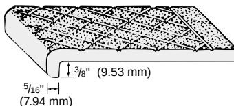
TYPE 101SP – Nose \frac{3}{8} " (9.53 mm). Chief use: as nosings on steel-pan concrete-filled stairs or superimposed on existing steps.
