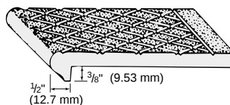
TYPE 102 – Nose \frac{1}{2} " x \frac{3}{8} " (12.7 mm x 9.53 mm). Chief use: as nosings on steel-pan stairs. Can also be used structurally with bent-plate risers.
