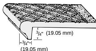
TYPE 103 – Nose \frac{3}{4} " x \frac{3}{4} " (19.05 mm x 19.05 mm). Chief use: as structural treads with bent-plate risers or as nosings full width of stair.
