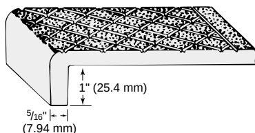
TYPE 116 – Nose depth 1" (25.4 mm) standard. Chief use: as nosings in concrete stairs where deeper lip is desirable.
