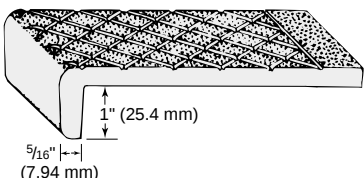
TYPE 116A – Nose depth 1" (25.4 mm) standard. Chief use: superimposed on existing steps for repair and modernization. Also see Type 500 on page 15.
