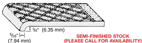
TYPE 101 – Nose \frac{1}{4} " (6.35 mm) lip. Chief use: as nosings in concrete stairs. Tread installed flush all around.
