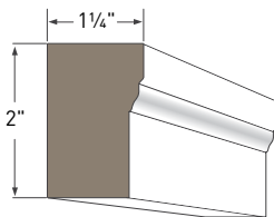
FLATBACK BRICK MOULD AZM-7526 Lengths: 17'
