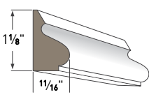
BASE CAP AZM-164 Length: 16'
