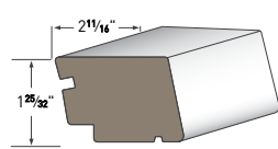
LARGE HISTORIC SILL AZM-7958 Length: 16'
