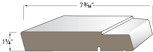
DOUBLE HUNG SILL AZM-7650 Length: 18'
