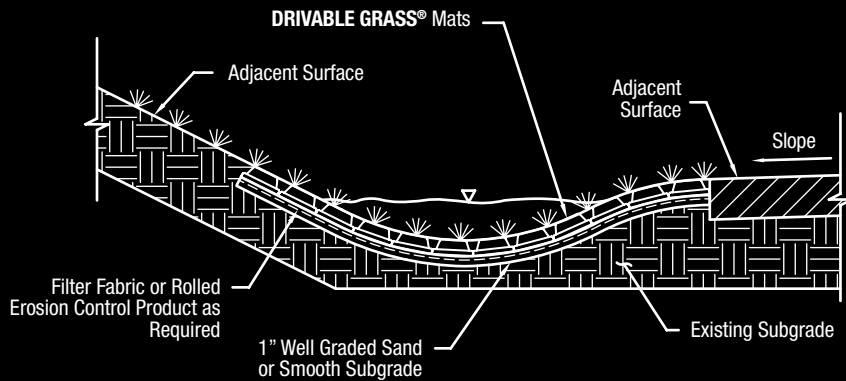
Typical Drainage Swale Detail
