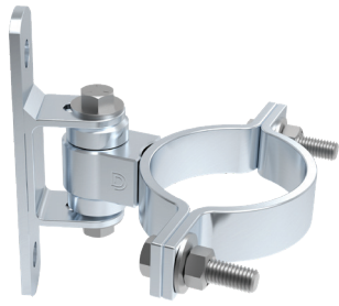
CI2051- 4" (102MM) ROUND BOLT-ON CI2053- 6" (152MM) ROUND BOLT-ON CI2054- 8" (203MM) ROUND BOLT-ON
