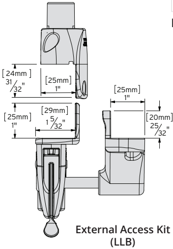
Round Post Model + EAK
