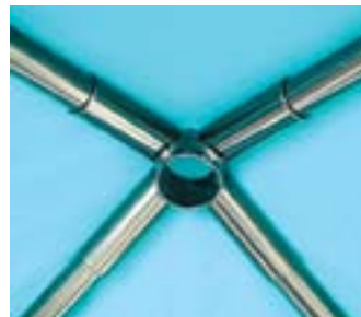
Underside center peak fitting, welded steel, built for quick and easy frame assembly.
