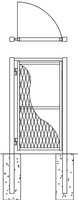
Pedestrian Swing Gate
