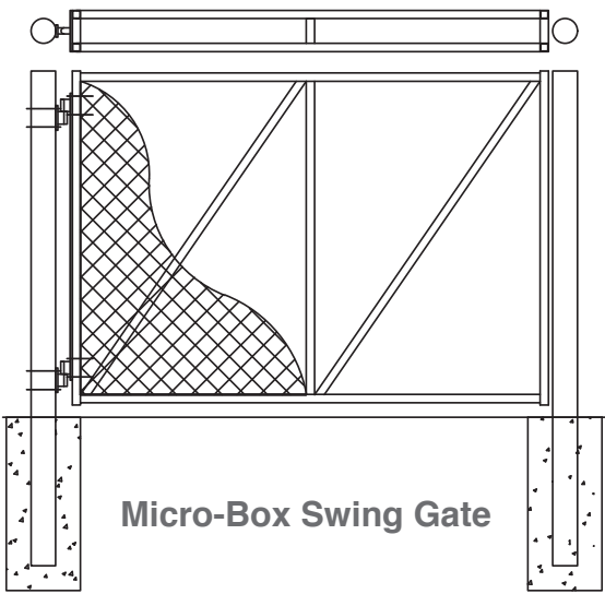
Pedestrian Swing Gate
