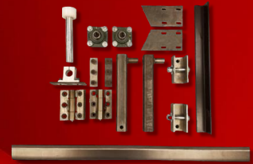
FLEXGUIDE FOLDING GATE KIT
