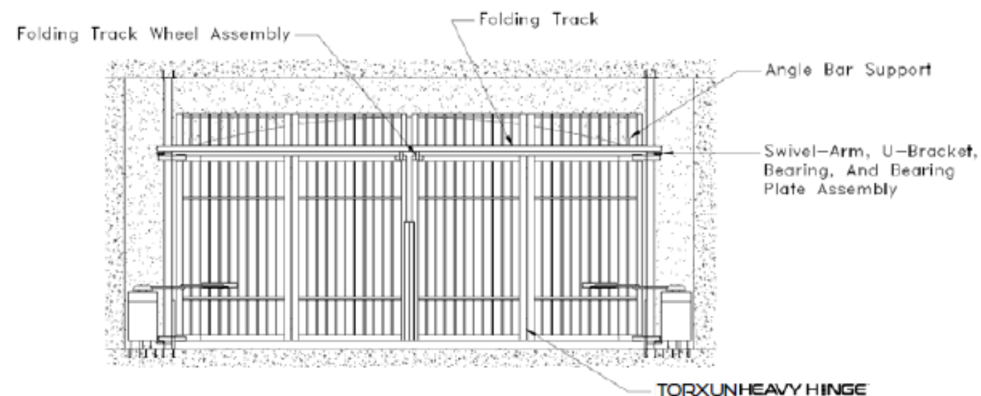
QUICKFOLD™ FLEXGUIDE™ Typical System
