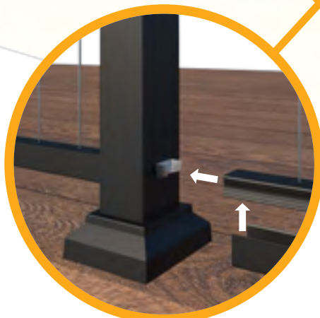
STRAIGHT CLIP BRACKET ASSEMBLE BELOW H-CHANNEL TO STRAIGHT CLIP AND BOTTOM SNAP TO BELOW H-CHANNEL
