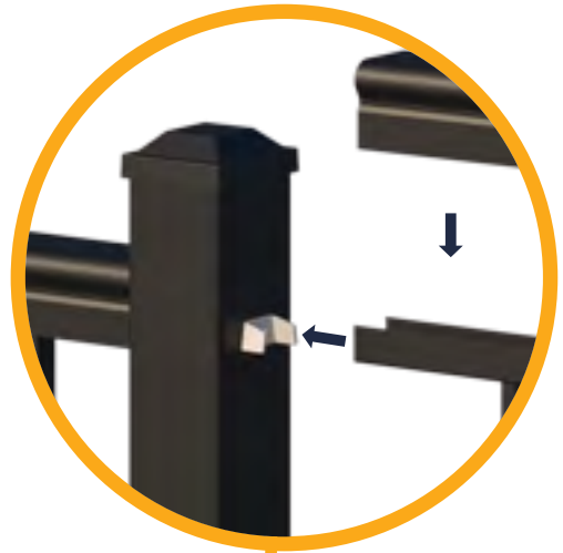
STRAIGHT CLIP BRACKET ASSEMBLE ABOVE H-CHANNEL TO STRAIGHT CLIP AND TOP RAIL ON TOP OF ABOVE H-CHANNEL
