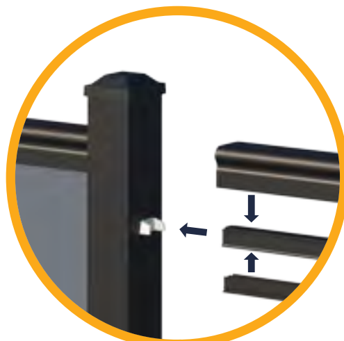
STRAIGHT CLIP BRACKET ASSEMBLE GLASS UPPER CHANNEL TO ALUMINUM POST
