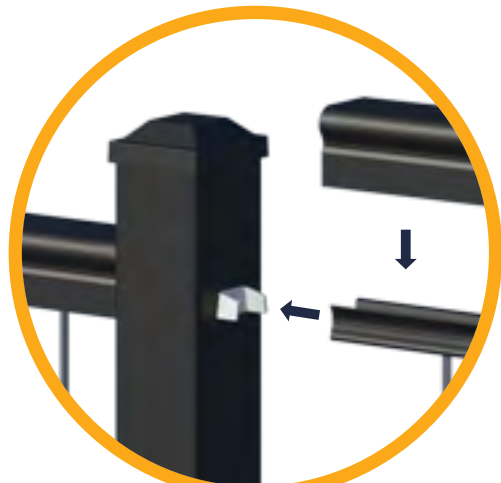
STRAIGHT CLIP BRACKET ASSEMBLE ABOVE H-CHANNEL TO STRAIGHT CLIP AND TOP RAIL ON TOP OF ABOVE H-CHANNEL
