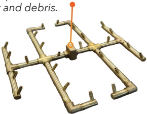
CROSSFIRE® Brass Burner
