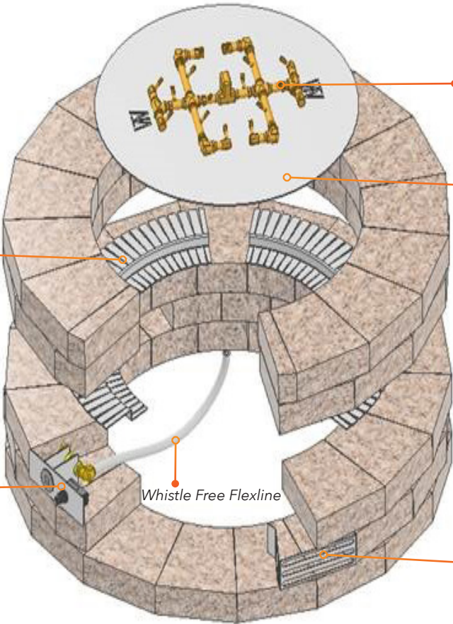
CROSSFIRE® Brass Burner
