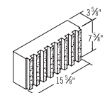
4x8x16 Split Face Eight Rib Fluted
