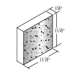
4x16x16 1F Solid
