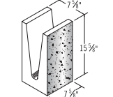
8x16x8 1F Deep Lintel BB*
