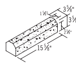
4x4x16 GFT DBL Chamfer
