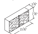
4x8x16 Split Face One Score
