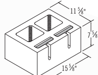
12x8x16 Acousta-Wal Type IV RF
