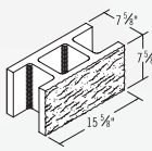
8x8x16 Fence Block
