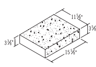
12x4x16 GFT Beveled Sill
