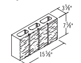
4x8x16 Split Face Three Score
