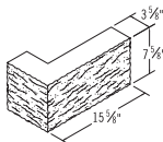
4x8x16 Split Face L-Corner
