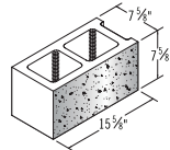
8x8x16 One Face
