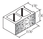
10x8x16 One Face
