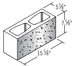
6x8x16 One Face
