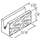
6x8x16 SF Solid Bottom Bond Beam
