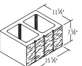
12x8x16 Split Face Three Score
