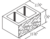
12x8x16 Split Face
