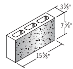
4x8x16 One Face
