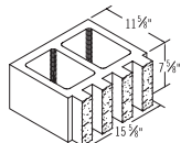
12x8x16 Split Face Four Rib Fluted
