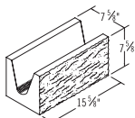
8x8x16 SF Solid Bottom Bond Beam
