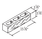
4x4x16 Split Face Half-High
