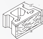
Keystone Compac III Victorian Split
