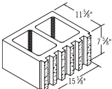
12x8x16 Split Face Six Rib Fluted
