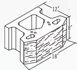
Keystone Compac III Tri-Plane
