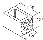
12x8x8 Split Face Half
