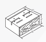
Versa-Lok Standard Unit
