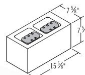
8x8x16 Icon Insulated*
