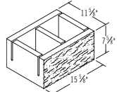
12x8x16 Split Face Knock Out Bond Beam
