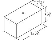
8x8x16 HP Solid (3/4" Hole)
