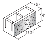
8x8x16 1F Knock Out BB*
