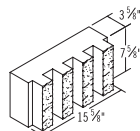
4x8x16 Split Face Four Rib Fluted
