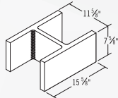
12x8x16 H Block
