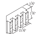
4x8x16 Split Face Four Rib Fluted Mitre
