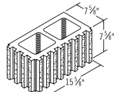
8x8x16 Split Face Eight Rib Fluted Corner
