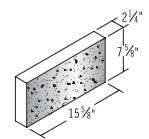
2 1/4x8x16 1F Solid
