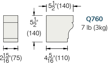
Cill Bracket
