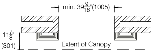
Georgian Door Surround Retrofit Q320 Tech Sheet: TL40
