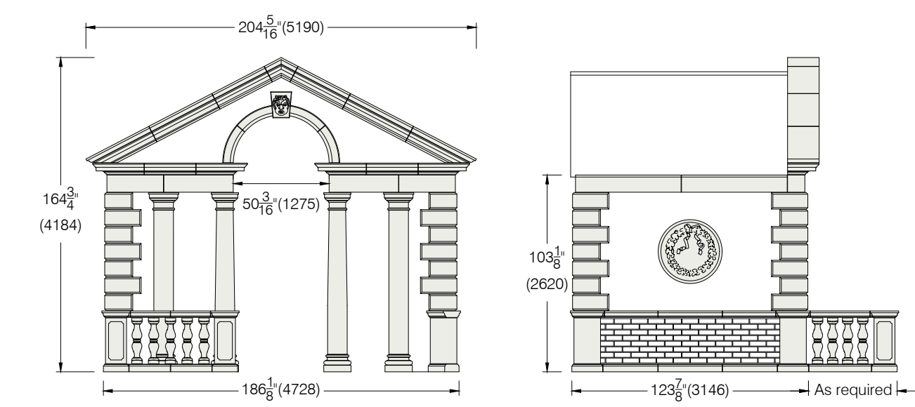
Venetian Folly L9400 Tech Sheet: T50, T51, T52
