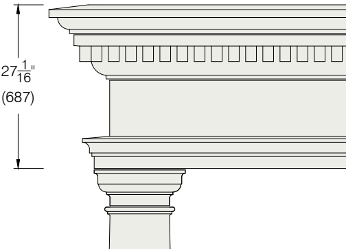
Portico B Tech Sheet: PT20, PT21
