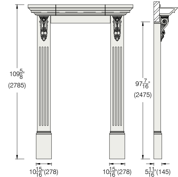
Traditional Door Canopy Retrofit Q335
