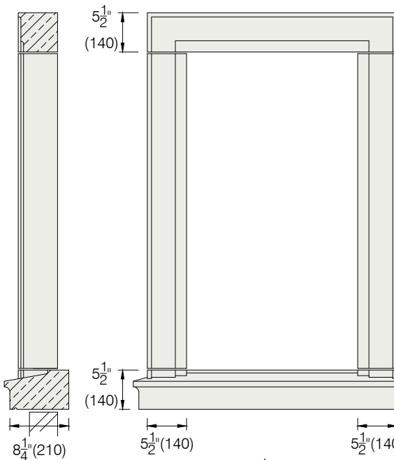
Cill Bracket
