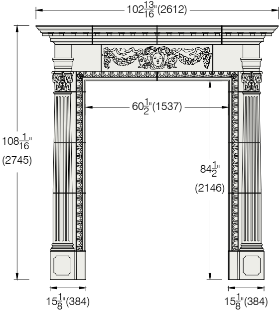
Built-in QU200 Tech Sheet: DS11
