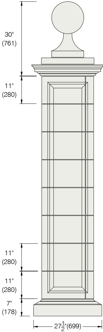
Gate Pier S120 Tech Sheet: M40
