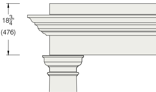
Portico D Tech Sheet: PT40, PT41
