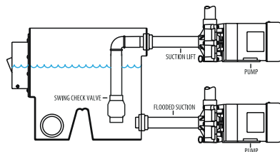
2" pump connection
