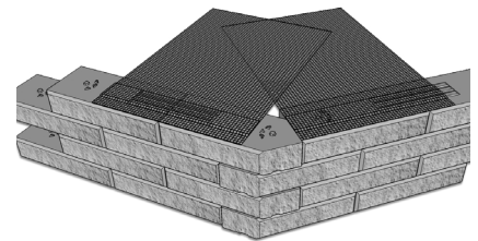
Reverse side of 435 Split Block
