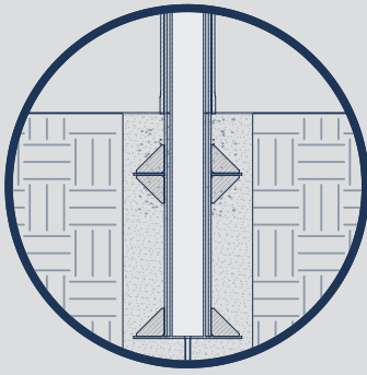
Deep Mount Bollard
