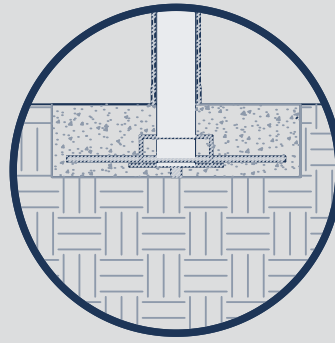
Shallow Mount Bollard
