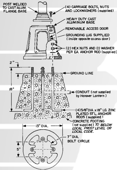
L Details for 316-317-318-319 320-321-755-758 posts.
