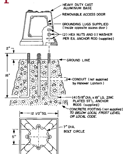
P Details for 400-402 posts.
