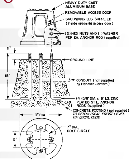
O Details for 401 posts.
