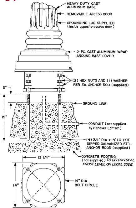
N Details for 294-295-296-297 posts.
