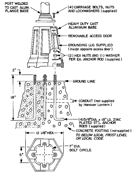
N Details for 294-295-296-297 posts.
