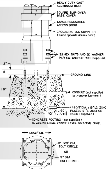
L Details for 316-317-318-319 320-321-755-758 posts.
