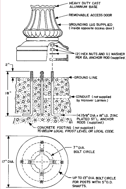
M Details for 303-304-305-306-307-308-311-751-754 posts.
