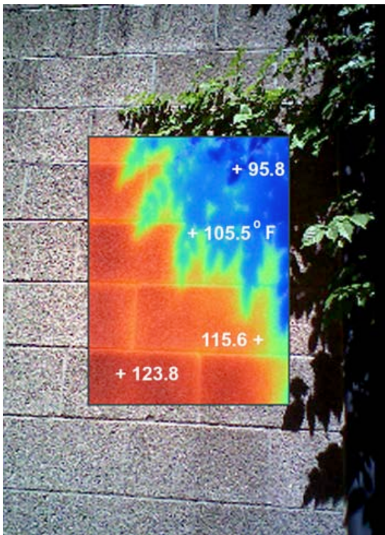
Infrared photography demonstrating temperatures on the building surface, Tempe, AZ
