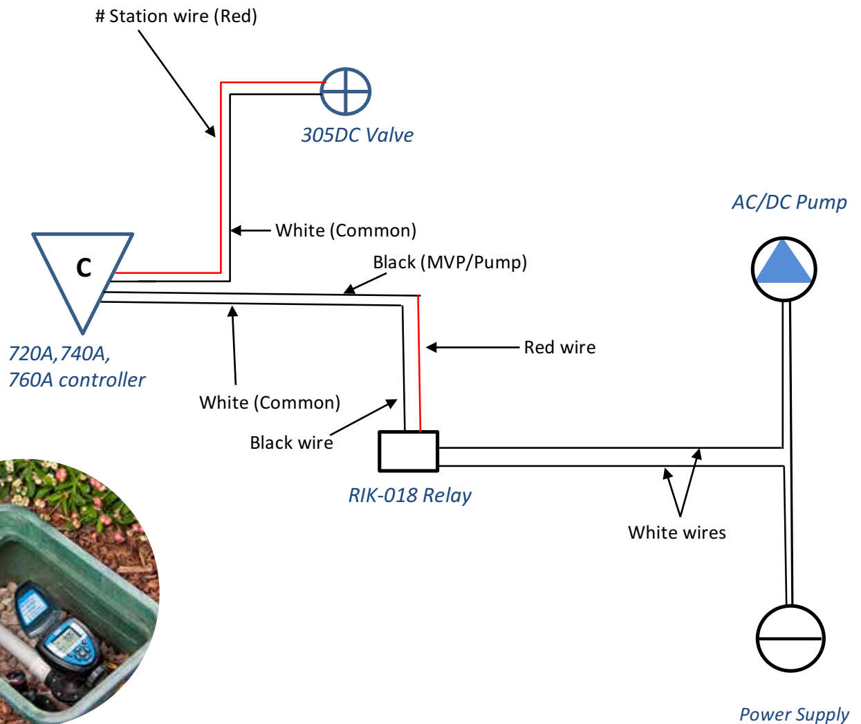
RIK-018 Wiring Diagram to 700A series Multi-Station DC Controllers
